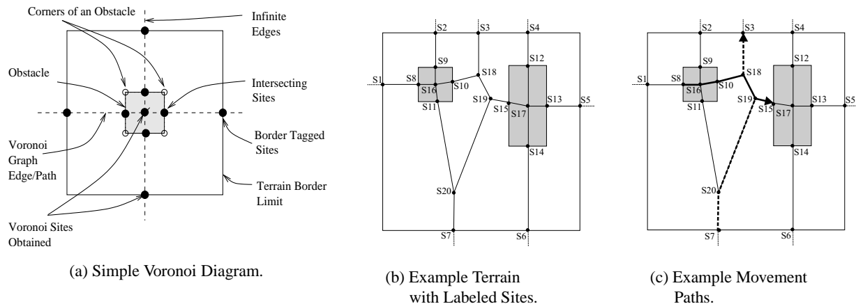
Figure 1: Examples of Voronoi graph, paths and movement.
