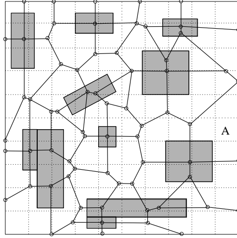
Figure 2: Simulated terrain.
