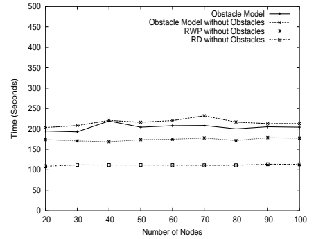
Figure 5: Average Link Duration.
