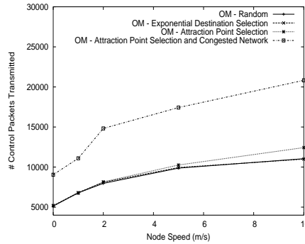
Figure 11: Control Packet Overhead.
