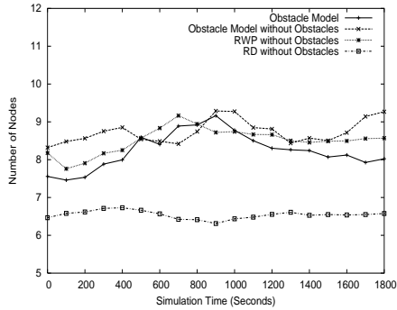
Figure 3: Node Density.
