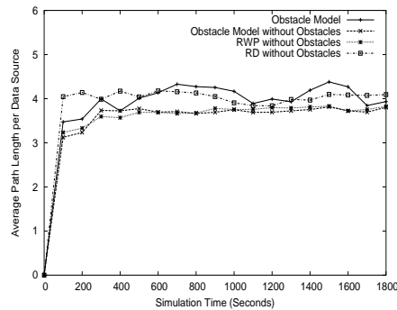
Figure 4: Path Length versus Time.
