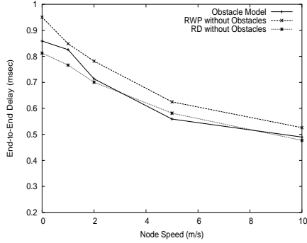
Figure 8: End-to-End Latency.
