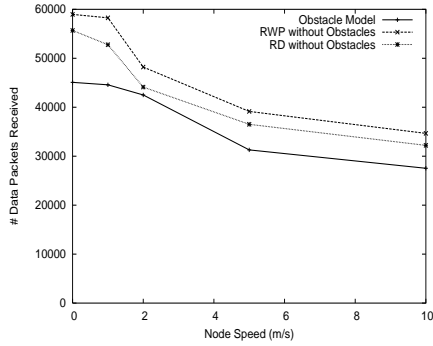
Figure 6: Data Packet Reception.
