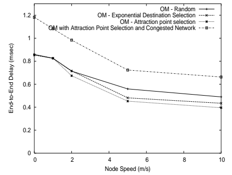
Figure 12: End-to-End Latency.
