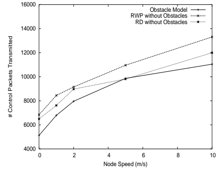
Figure 7: Control Packet Overhead.
