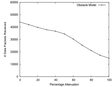
Figure 9: Data Packet Reception versus Signal Attenuation Percentage.
