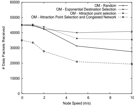
Figure 10: Data Packet Reception.
